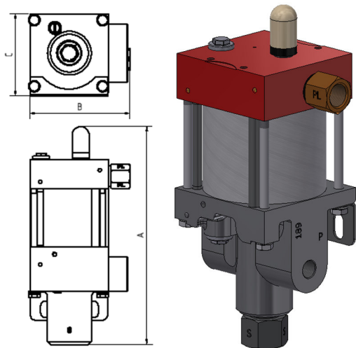
MO189 single acting, single air drive head (Standard= Bottom inlet)
