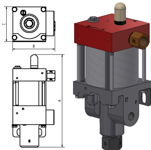
MO72 Single acting, single air drive head (Standard= Bottom inlet)
