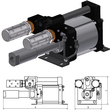
GX100 double acting, single air drive head (Standard= Bottom inlet)
