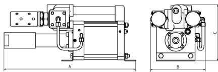
GX35 double acting, single air drive head (Standard= Bottom inlet)
