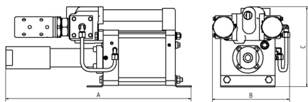
GX60 double acting, single air drive head (Standard= Bottom inlet)
