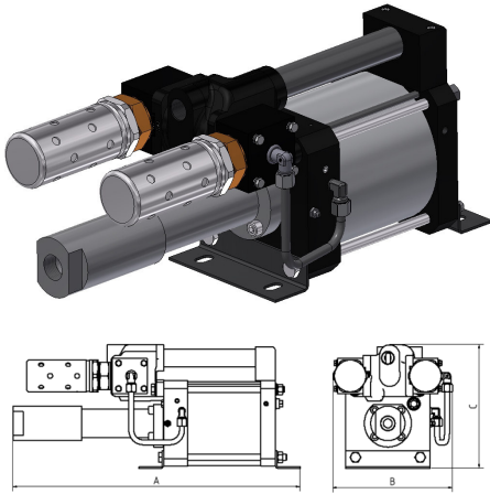
GX170 double acting, single air drive head (Standard= Bottom inlet)
