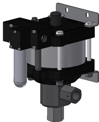
G25 (L) single acting, single air drive head (Standard= Bottom inlet)
