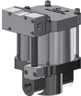
S150 single acting, single air drive head
