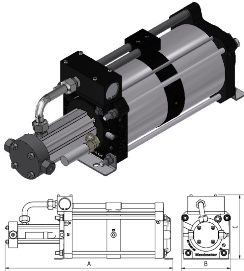
DLE 15-1-2 single acting, single air drive head; single stage
