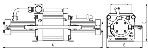
DLE 15-30 single acting, single air drive head two stages
