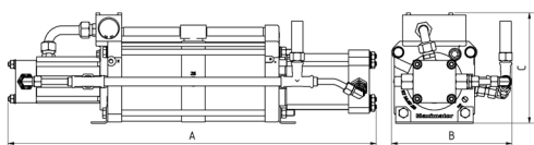
DLE 2-5-2 single acting, double air drive head two stages
