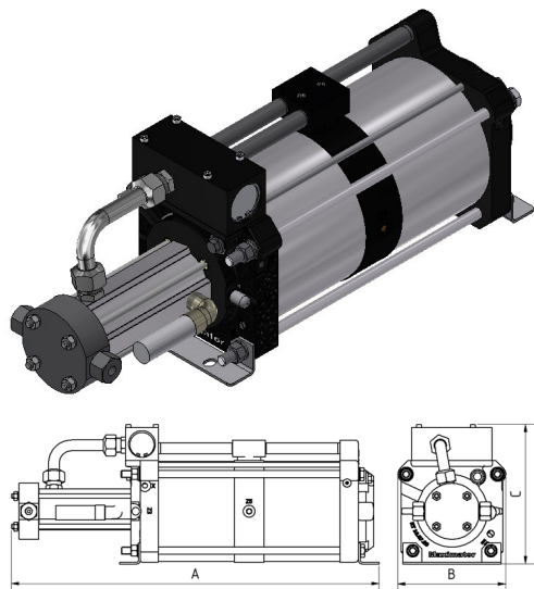
DLE 30-1-2 single acting, single air drive head single stage
