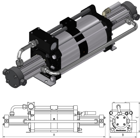
DLE 30-2 double acting, double air drive head single stage
