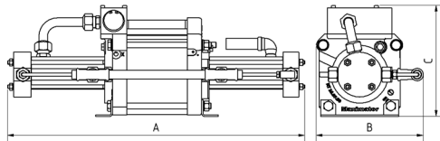
DLE 30-75 single acting, single air drive head two stages
