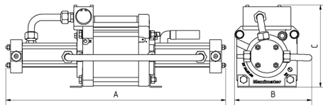
DLE 75 double acting, single air drive head single stage
