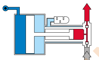
Working principle ROB 22
