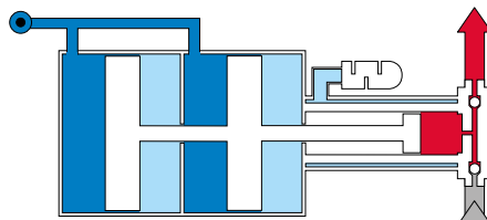
Working principle DLE 15-1-2
