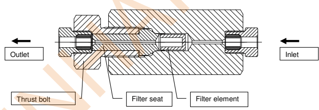
Figure 14: Structure of a cup/type filter
